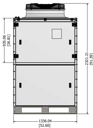
VISTA FRONTAL
